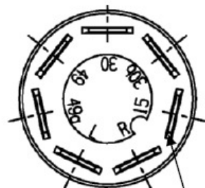
plug connection
