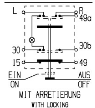
Circuit diagram
